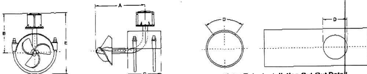
Meter Tube Installation Cut-Out Detail
